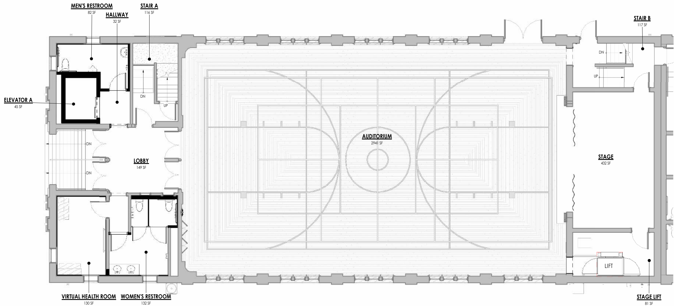
1 FLOOR PLAN - LEVEL 1
