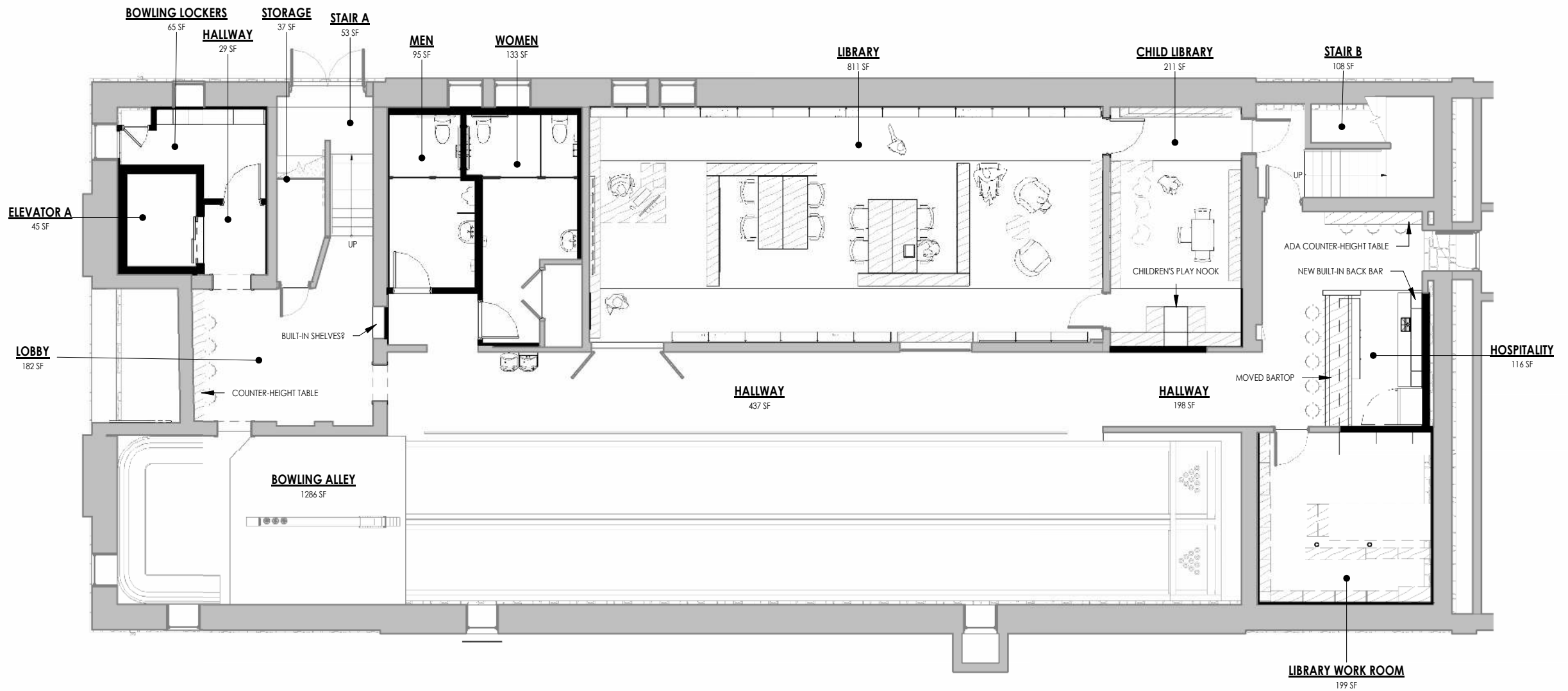
1 FLOOR PLAN - LEVEL 0
