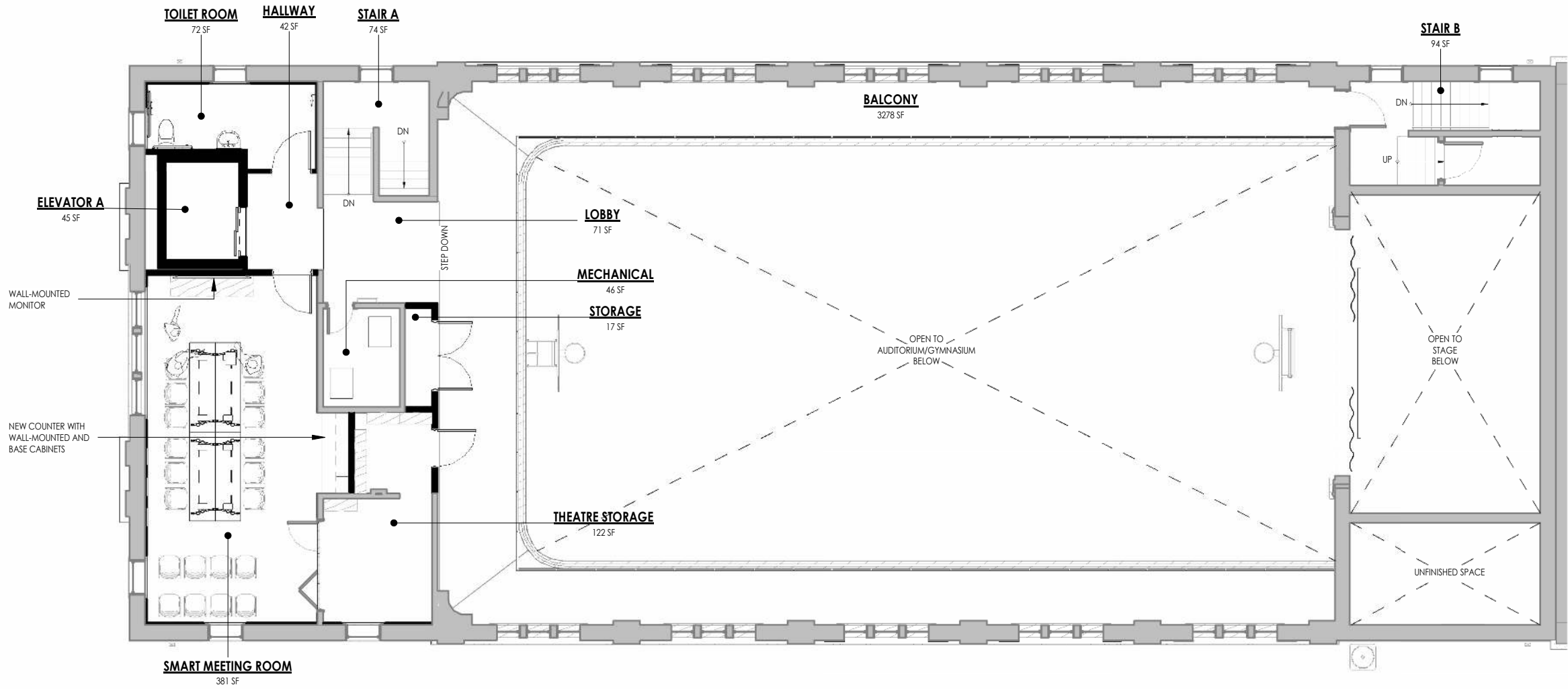
1 FLOOR PLAN - LEVEL 2
